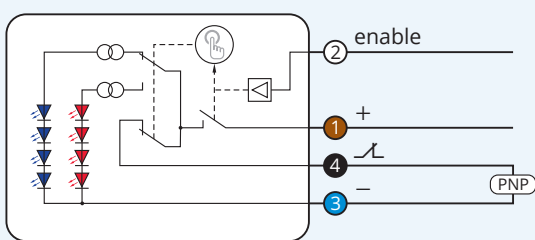
Pinout
