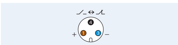
Pinout
