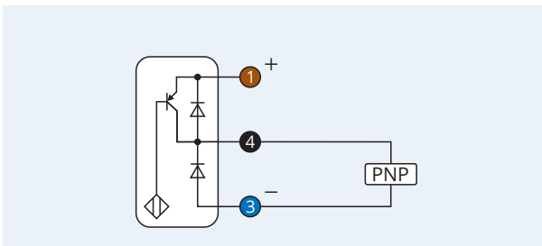
Pinout
