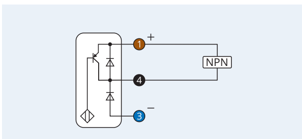
Pinout
