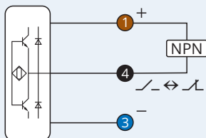
Pinout
